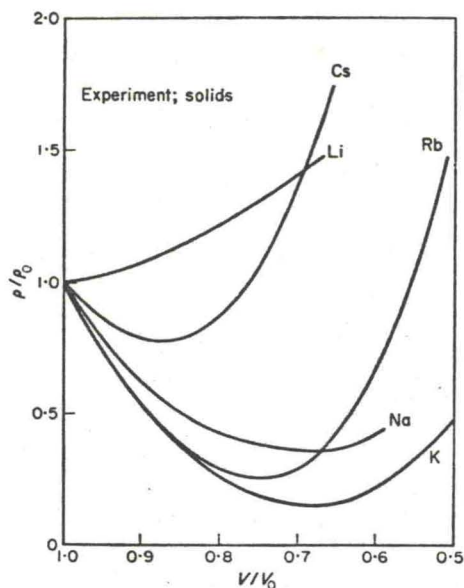
FIG. 23. Bridgman's results of the alkali metals at 0° C. The curves show relative resistance versus relative volume.
